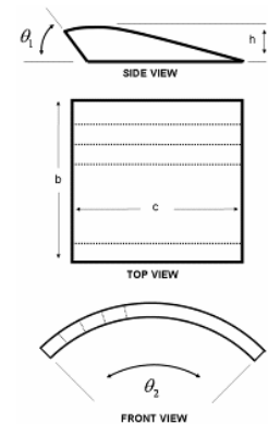
Fig. 3 Canopy geometry.
