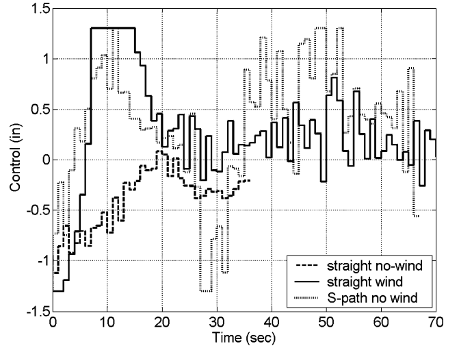
Fig. 8 Control.
