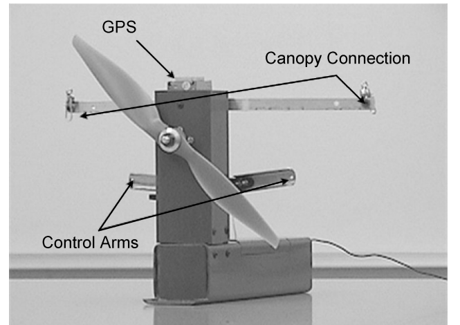
Fig. 1 Payload.
